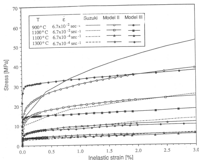
Fig. 16—Typical tensile test curves calculated with models II and III using initial structure constant of 1.54 compared with Suzuki data. [35]
