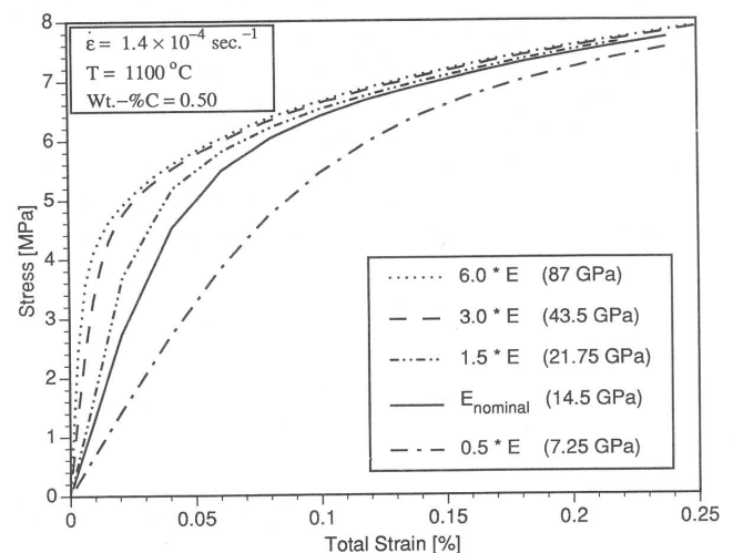
Fig. 1—Effect of variations in elastic modulus on shape of a typical stress-strain curve (model II; E_{\text{nominal}} = 14.5 GPa).
