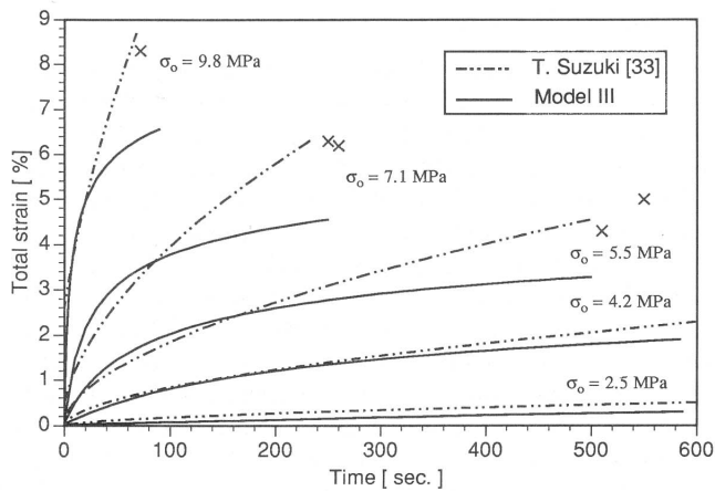
Fig. 12—Creep test curves calculated with model III at 1300 °C (compared with Suzuki [33] data; X denotes recrystallization).
