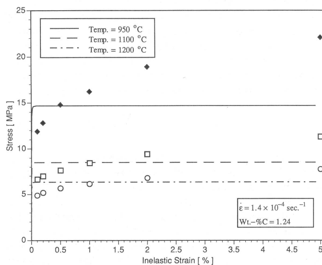
Fig. 2—Tensile test stress-strain curves calculated with model IA at different temperatures (compared with experimental tensile test data from Wray [32] ).
