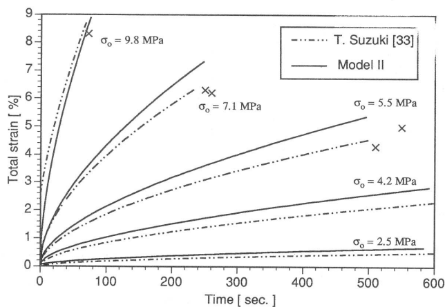
Fig. 6—Effect of stress on creep test strain-time response of model II at 1300 °C (compared with Suzuki data; [33] X denotes recrystallization).
