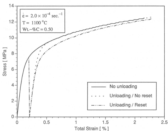
Fig. 19—Tensile test curves calculated with model II for unloading at 0.2 pct strain and reloading at the previous strain rate.
