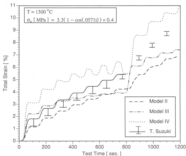
Fig. 22—Sinusoidal loading response of models II through IV compared with experimental data for 0.19 pct C steel, [33] whose range is indicated by I bars.
