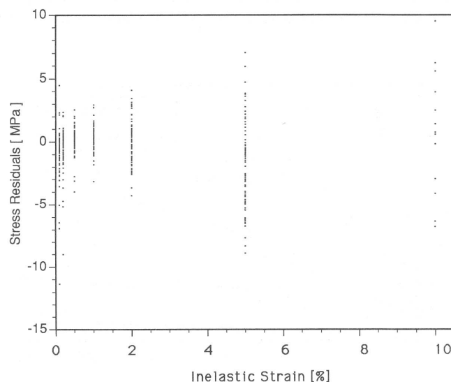
Fig. 11—Distribution of errors in model III stress predictions plotted against inelastic strain.
