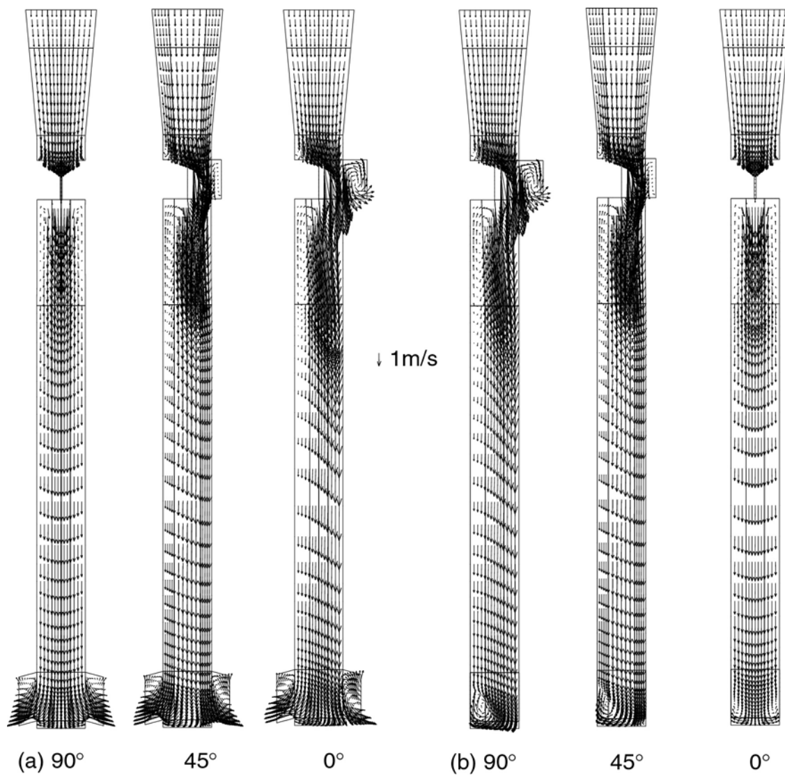
Figure 3 Flow field at the center planes for different gate orientations (a) center plane parallel to wide face (b) center plane parallel to narrow face ( V_C=1\text{m/min} , Q_G=10\text{SLPM} , f_1=16\% , F_L=50\% ,)
