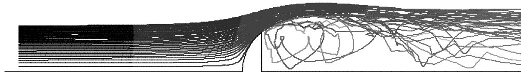
Figure 10 Inclusion trajectories in low turbulence ( d_b=100\text{mm} , d_p=100\mu\text{m} , k=10^{-6}\text{m}^2/\text{s}^2 )
