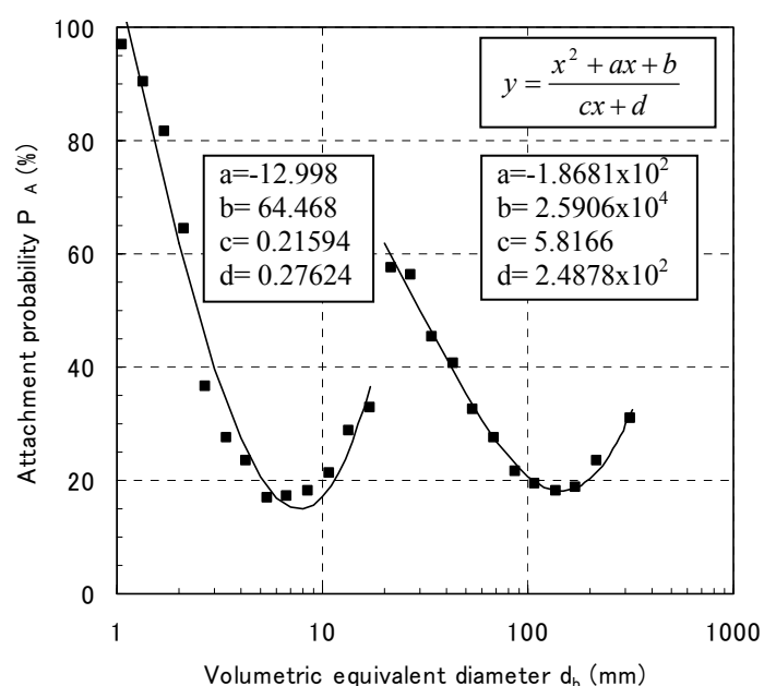
Figure 13 Fitting curve of attachment probability for d_p=100\mu\text{m} and k=0.1\text{m}^2/\text{s}^2
