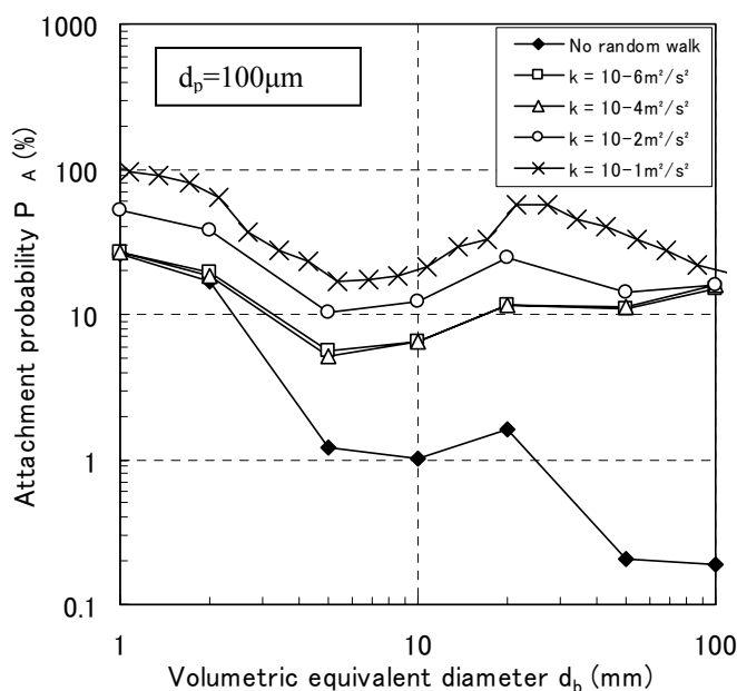
Figure 12 Particle attachment probability with turbulent random motion
