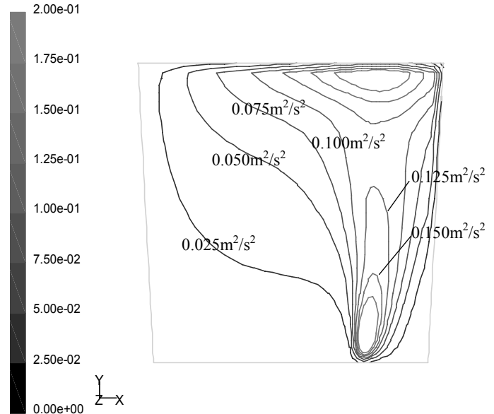
Figure 9 Calculated turbulent kinetic energy distribution (FLUENT output)
