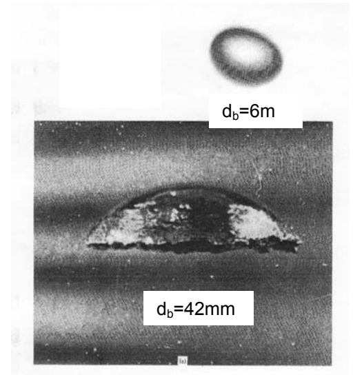
Figure 2. The shape of air bubbles in water [9]
