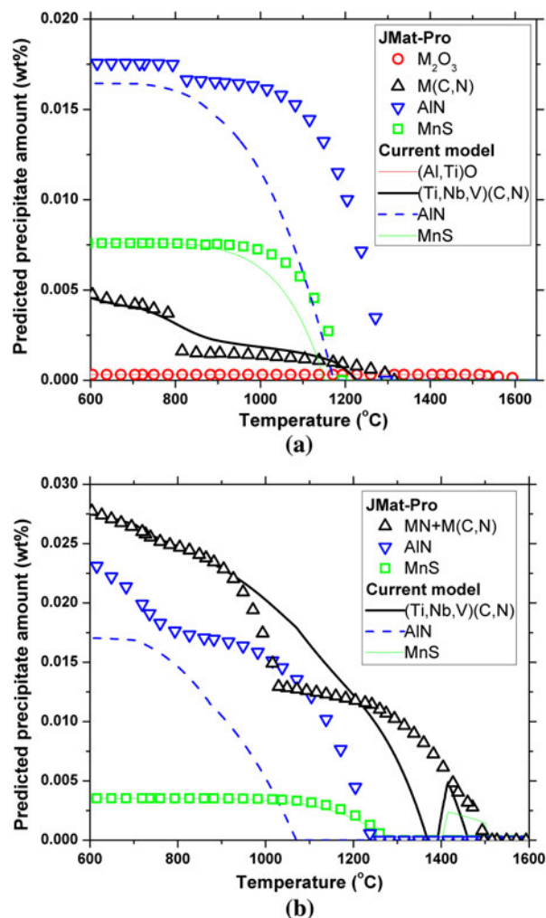
Fig. 5—Comparison of precipitate calculations by software JMat-Pro and the current model: (a) 1004 LCAK steel and (b) 1006Nb HSLA steel.
