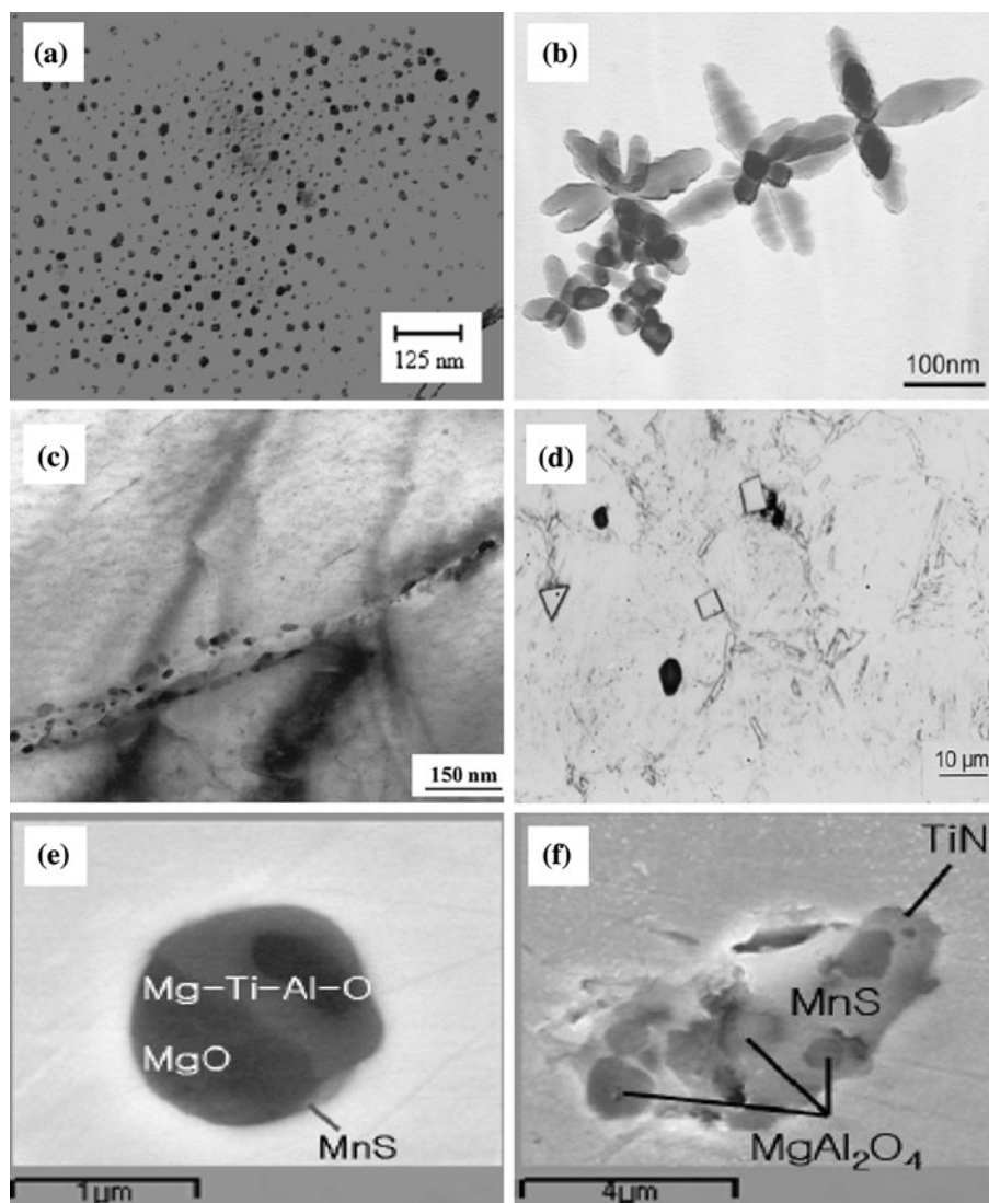
Fig. 1—Example precipitates in microalloyed steels: (a) fine spherical AlN, [2] (b) cruciform (Ti,V)N after equalization at 1373 K (1100 °C), [3] (c) (Ti,Nb)C on grain boundaries, [4] (d) cubic TiN on grain boundaries, [5] and (e) and (f) coarse complex multiple precipitates by heterogeneous nucleation. [6]
