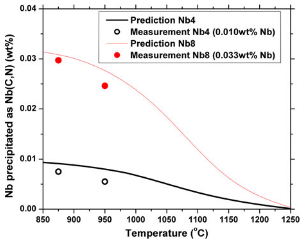
Fig. 6—Comparison of predicted amounts of Nb precipitation with experimental measurements at different temperatures (Table V steels [71] ).
