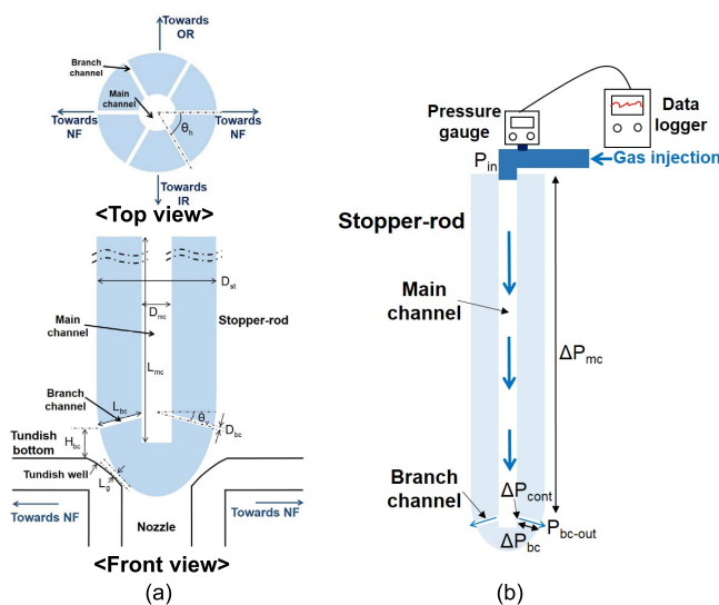
Fig. 2. (a) Schematic of the stopper-rod with multi-channels for gas injection, (b) gas injection through the stopper-rod and measurement of gas pressure in the water model. (Online version in color.)
