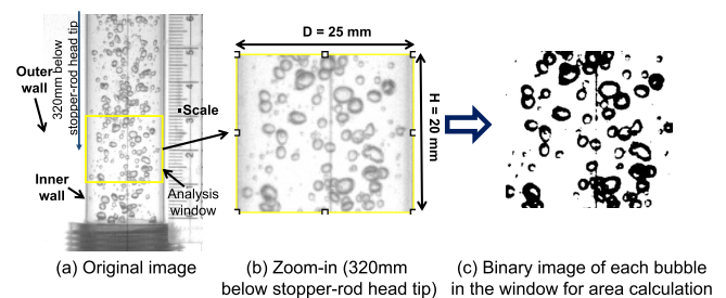
Fig. 3. Bubble size image analysis. (Online version in color.)
