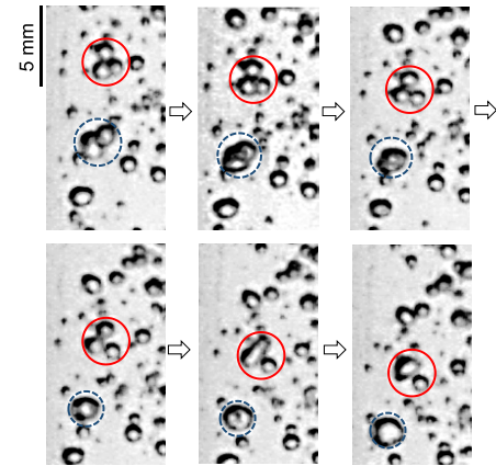
Fig. 12. Example of bubble coalescence in the nozzle region 150–160 mm below the stopper-rod head tip (833 \mu s between the snapshots): 35.0 LPM (water) and 0.2 LPM (air). (Online version in color.)
