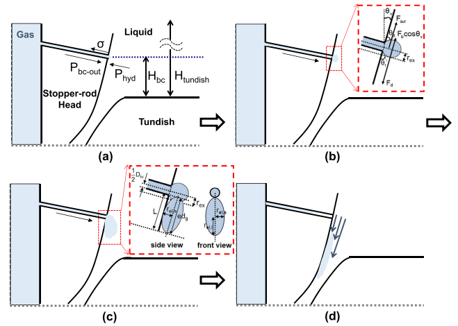
Fig. 4. Bubble formation mechanism: (a) initiation, (b) expansion, (c) elongation, and (d) detachment. (Online version in color.)
